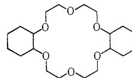
dicyclohexyl-18-crown-6 ether
